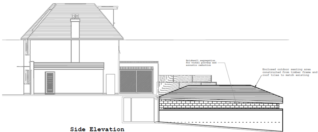
Side Elevation
