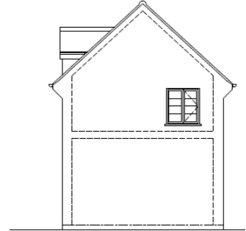
SIDE ELEVATION (North East)
