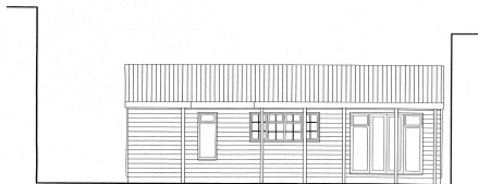
North-East Elevation
