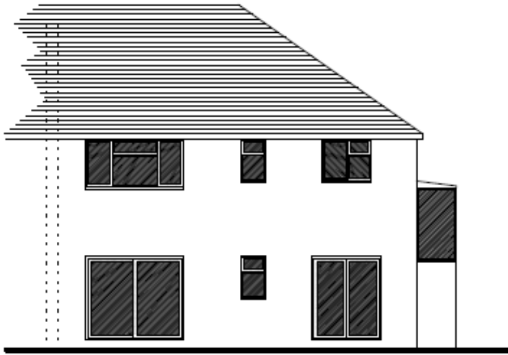
Rear Elevation
